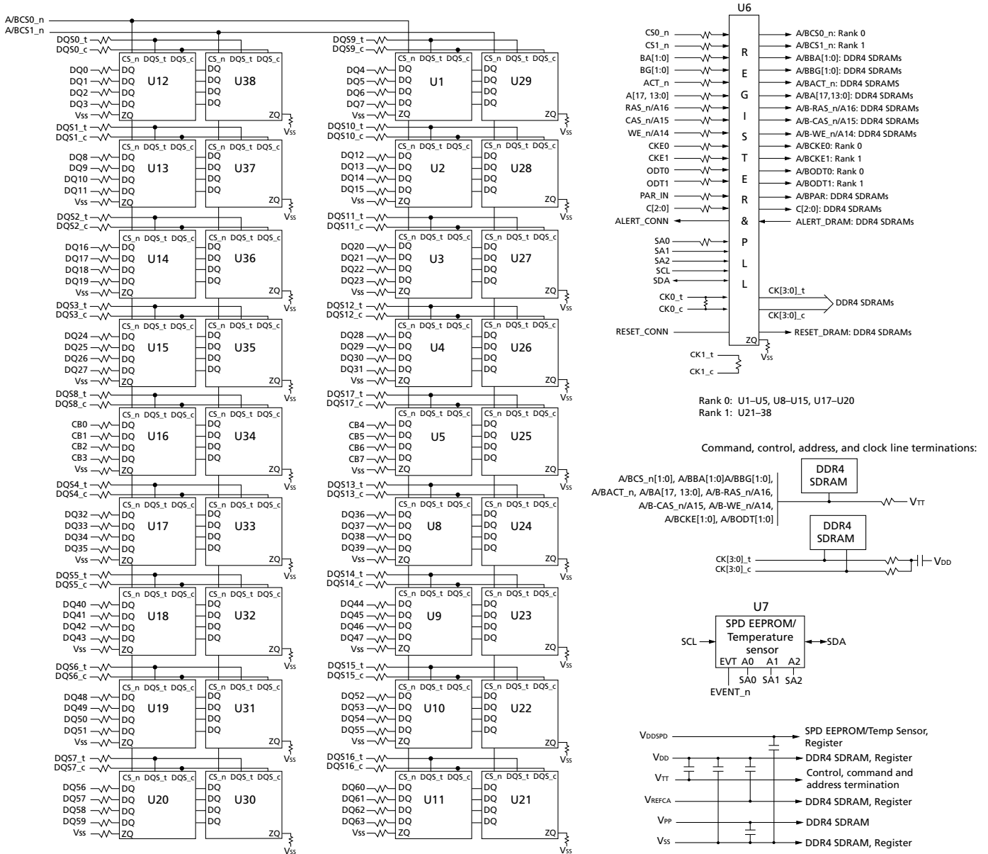
Figure 3: Functional Block Diagram (R/C-B1, PCB 1798, PCB 1870)
