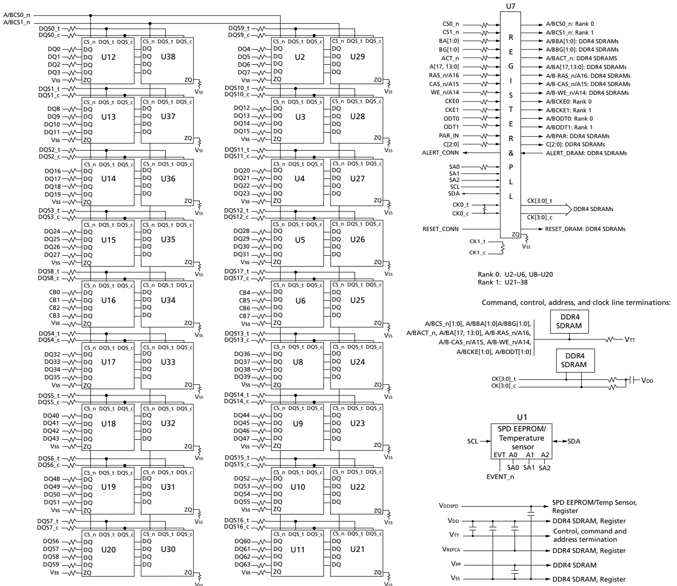
Figure 4: Functional Block Diagram (R/C-B2, PCB 1971, PCB 2364, PCB 2436, PCB 2893)
