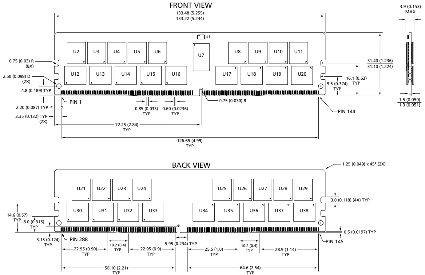
Figure 6: 288-Pin DDR4 RDIMM (R/C-B2, PCB 1971, PCB 2364, PCB 2463, PCB 2893)
